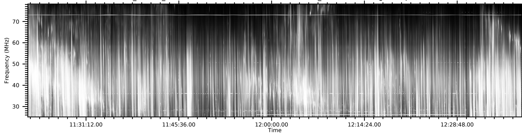
20240522_112100_BST - NW - Beam ana: 0 - Beam num: 0 - SUN_TRACKING - histogram-equalized data
