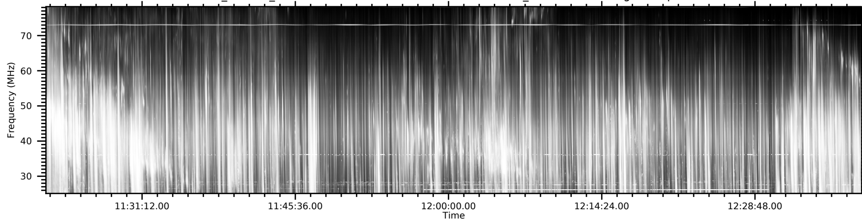
20240522_112100_BST - NE - Beam ana: 0 - Beam num: 0 - SUN_TRACKING - histogram-equalized data
