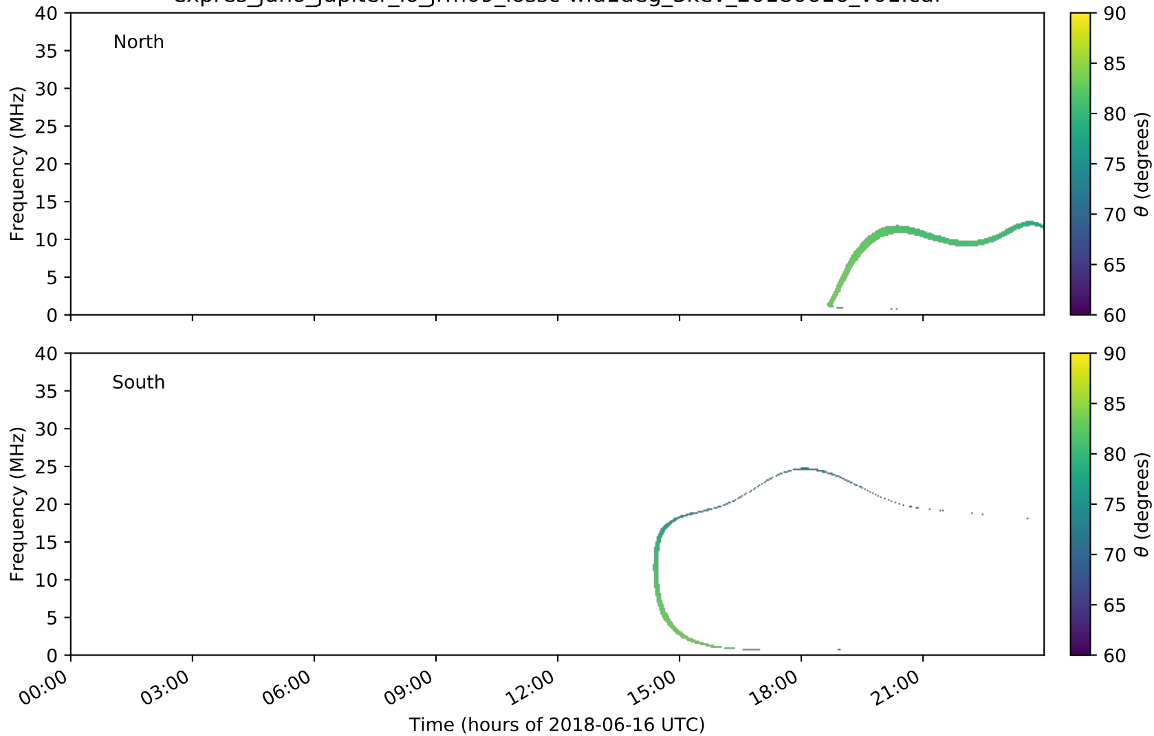
expres_juno_jupiter_io_jrm09_lossc-wid1deg_3kev_20180616_v01.cdf
