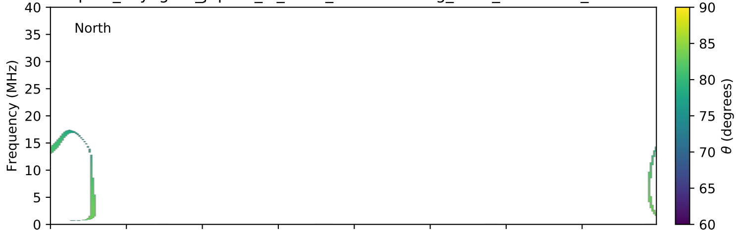
expres_voyager1_jupiter_io_isaac_lossc-wid1deg_3kev_19790317_v01.cdf
