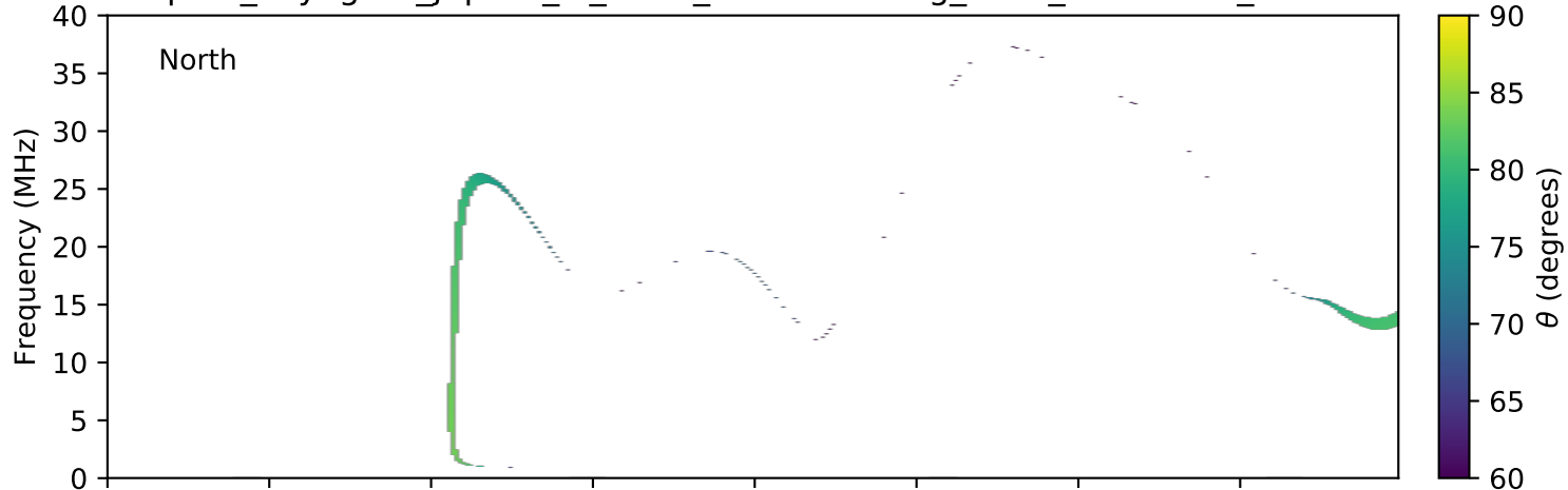
expres_voyager1_jupiter_io_isaac_lossc-wid1deg_3kev_19790316_v01.cdf
