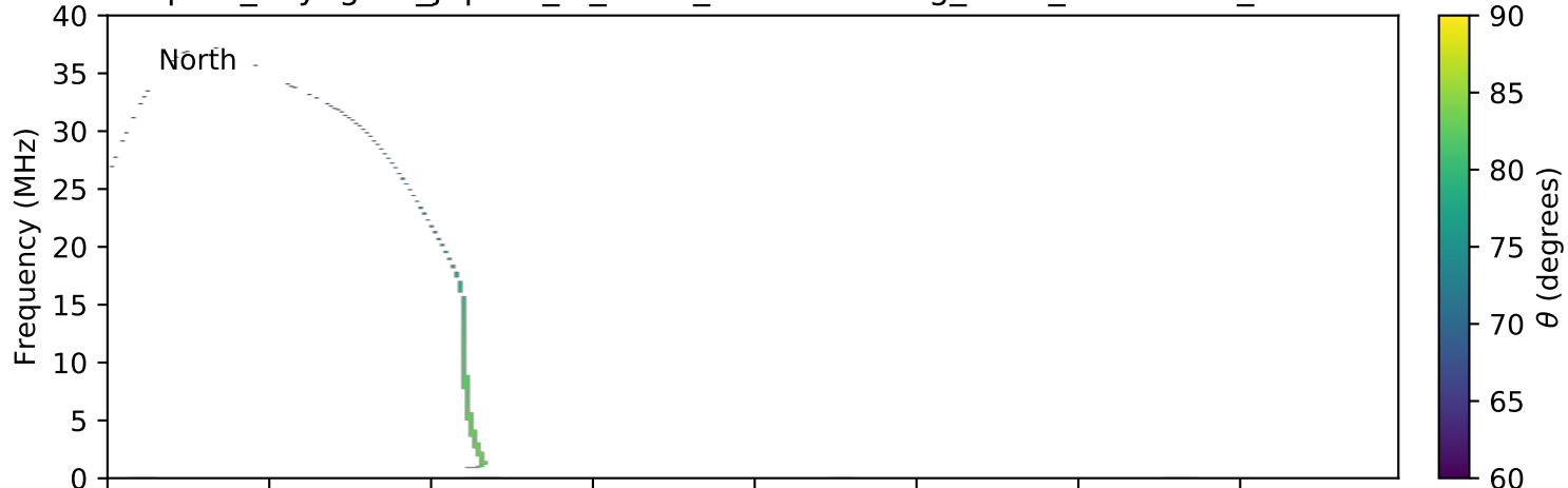
expres_voyager1_jupiter_io_isaac_lossc-wid1deg_3kev_19790315_v01.cdf
