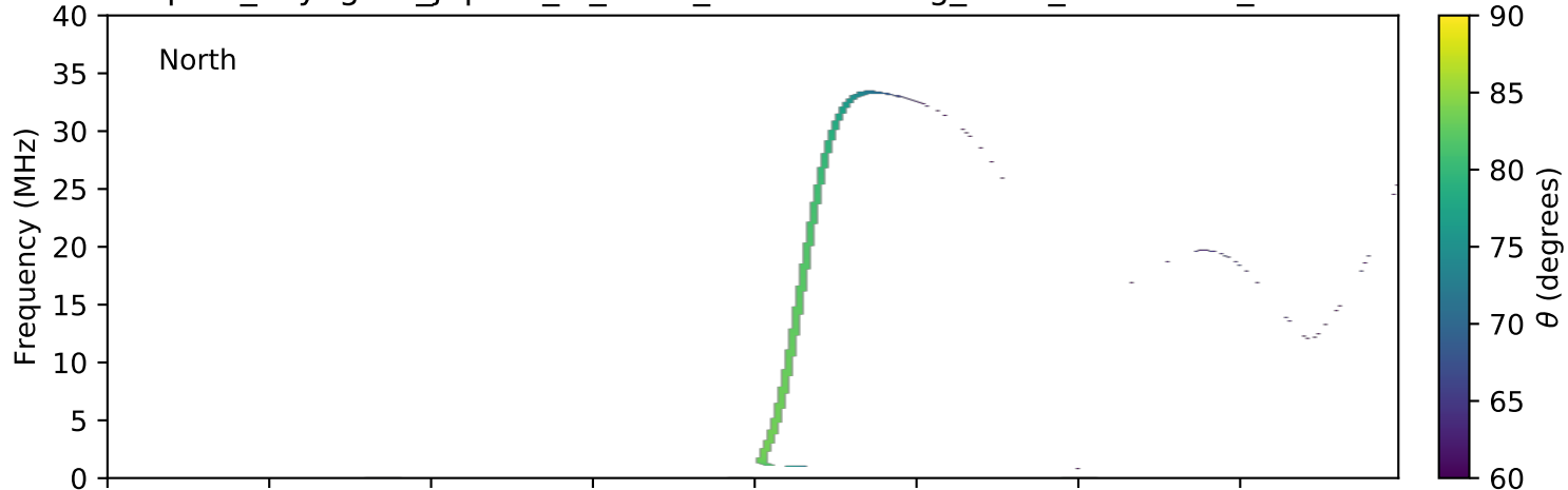
expres_voyager1_jupiter_io_isaac_lossc-wid1deg_3kev_19790314_v01.cdf
