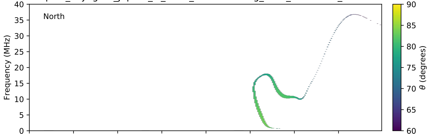
expres_voyager1_jupiter_io_isaac_lossc-wid1deg_3kev_19790312_v01.cdf
