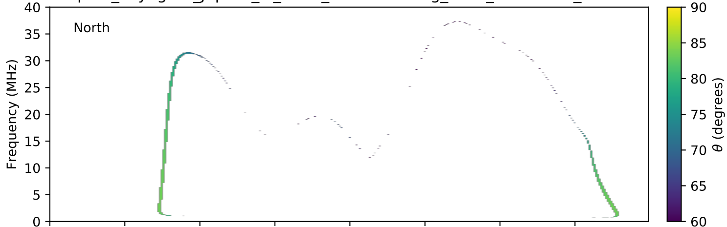
expres_voyager1_jupiter_io_isaac_lossc-wid1deg_3kev_19790309_v01.cdf
