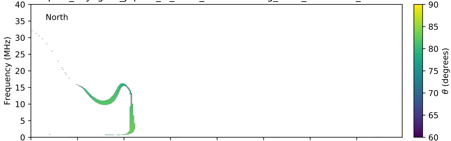
expres_voyager1_jupiter_io_isaac_lossc-wid1deg_3kev_19790306_v01.cdf
