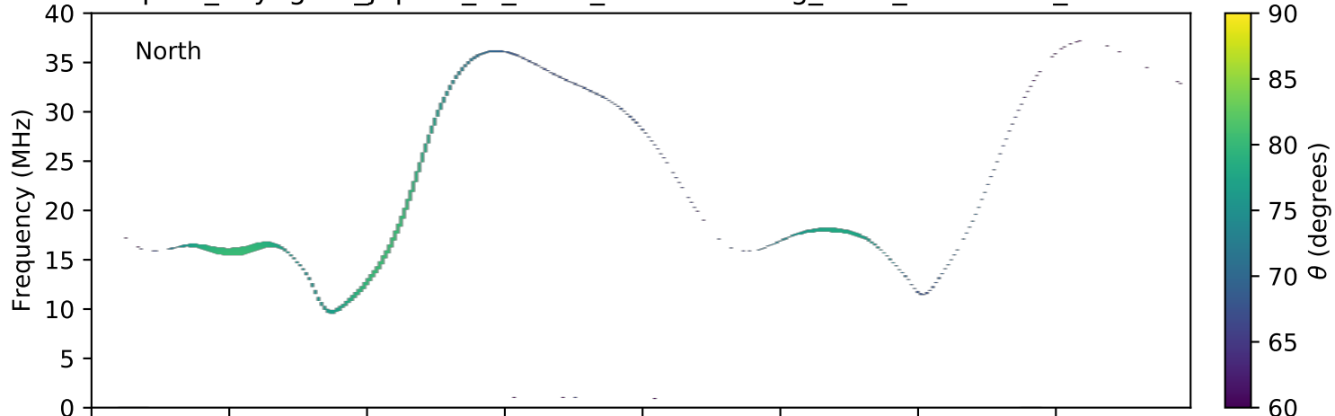
expres_voyager1_jupiter_io_isaac_lossc-wid1deg_3kev_19790305_v01.cdf
