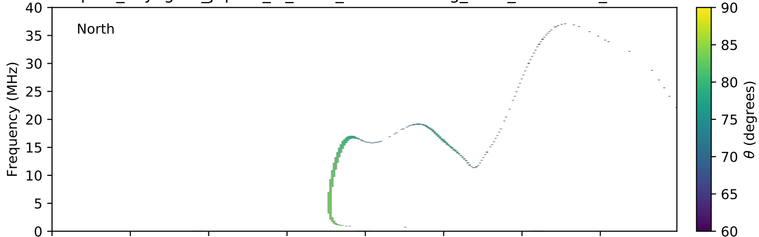
expres_voyager1_jupiter_io_isaac_lossc-wid1deg_3kev_19790304_v01.cdf
