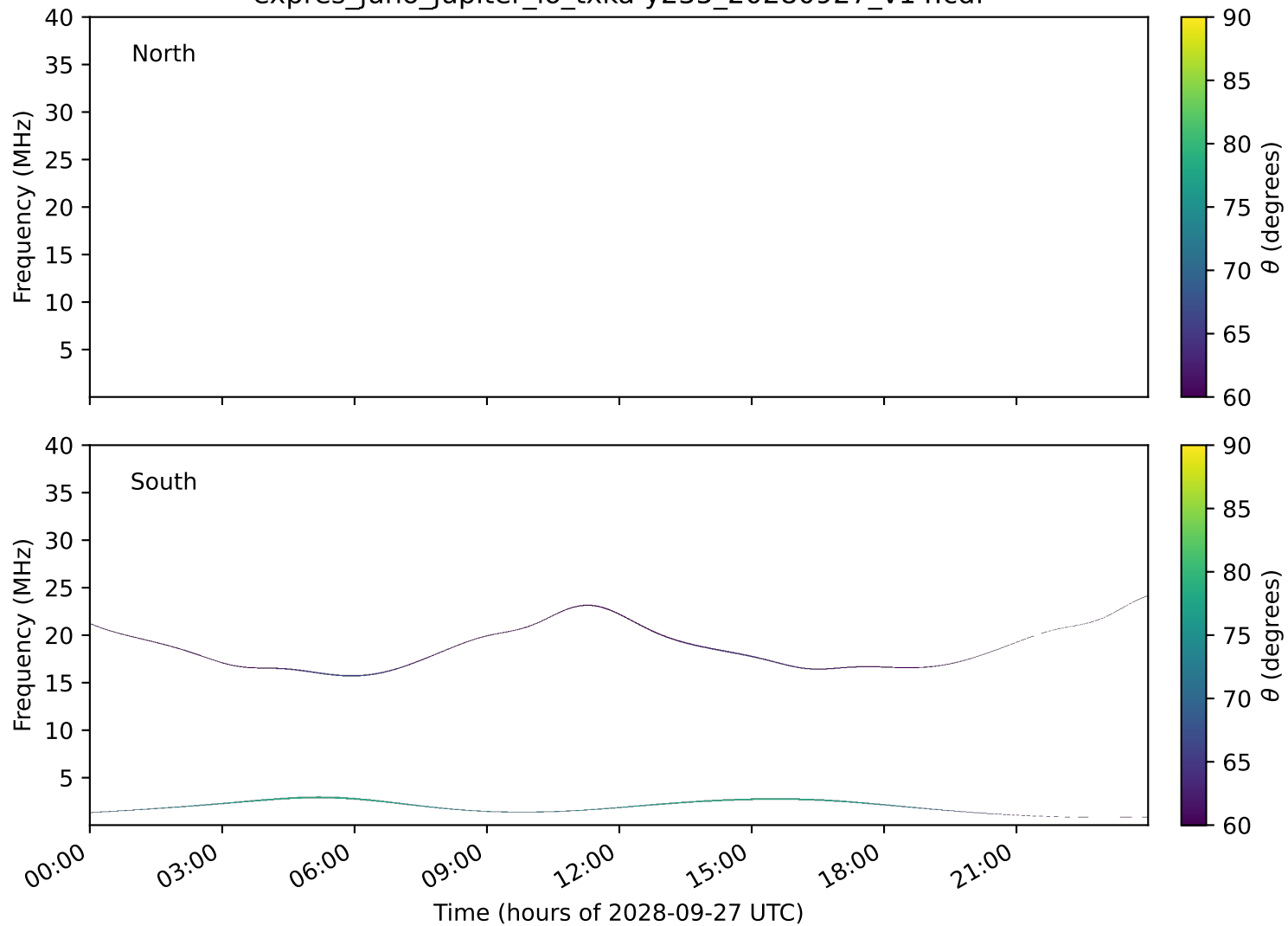
expres_juno_jupiter_io_txka-y235_20280927_v14.cdf
