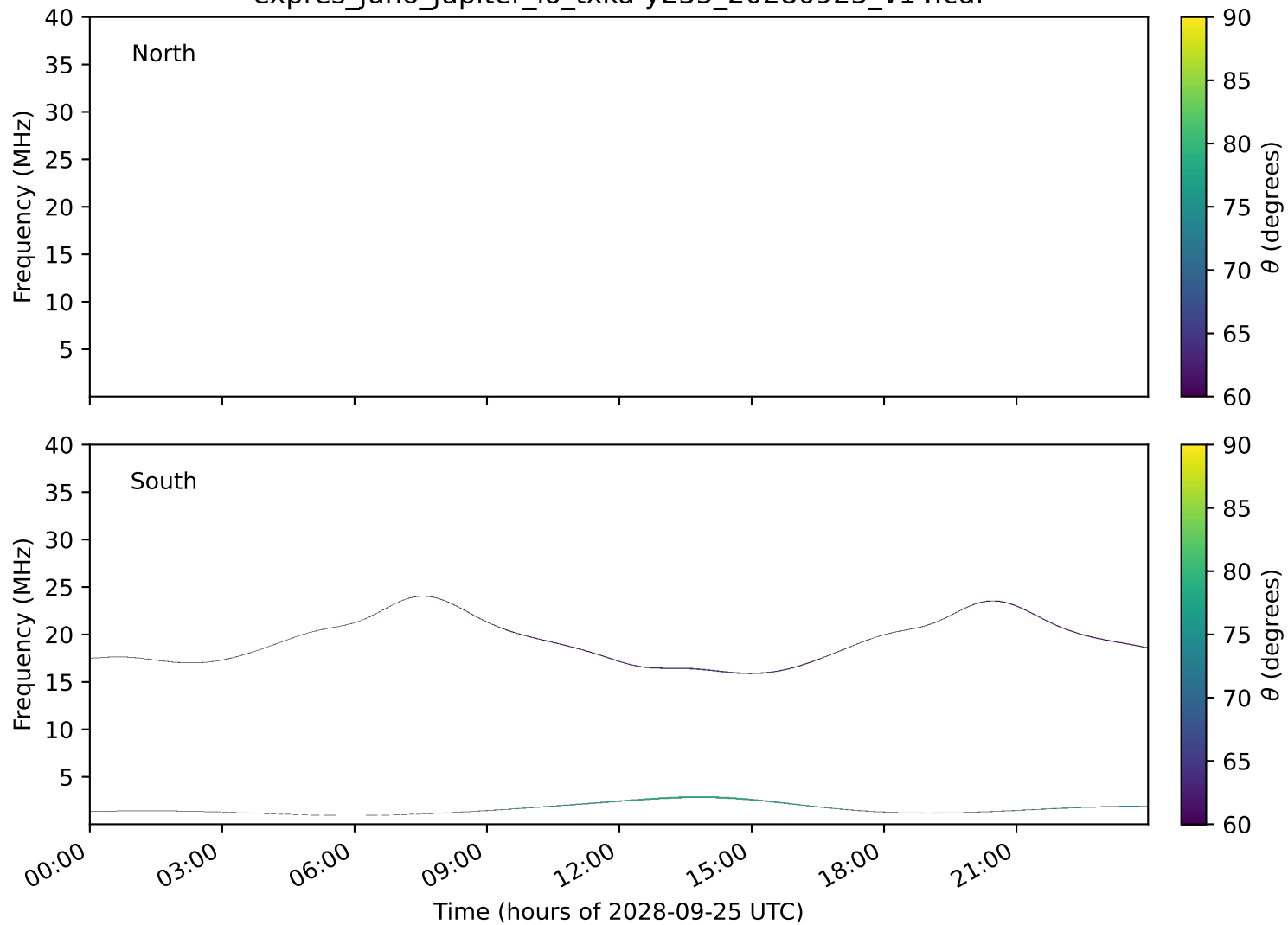
expres_juno_jupiter_io_txka-y235_20280925_v14.cdf
