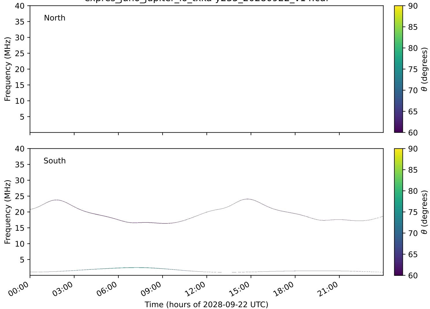
expres_juno_jupiter_io_txka-y235_20280922_v14.cdf
