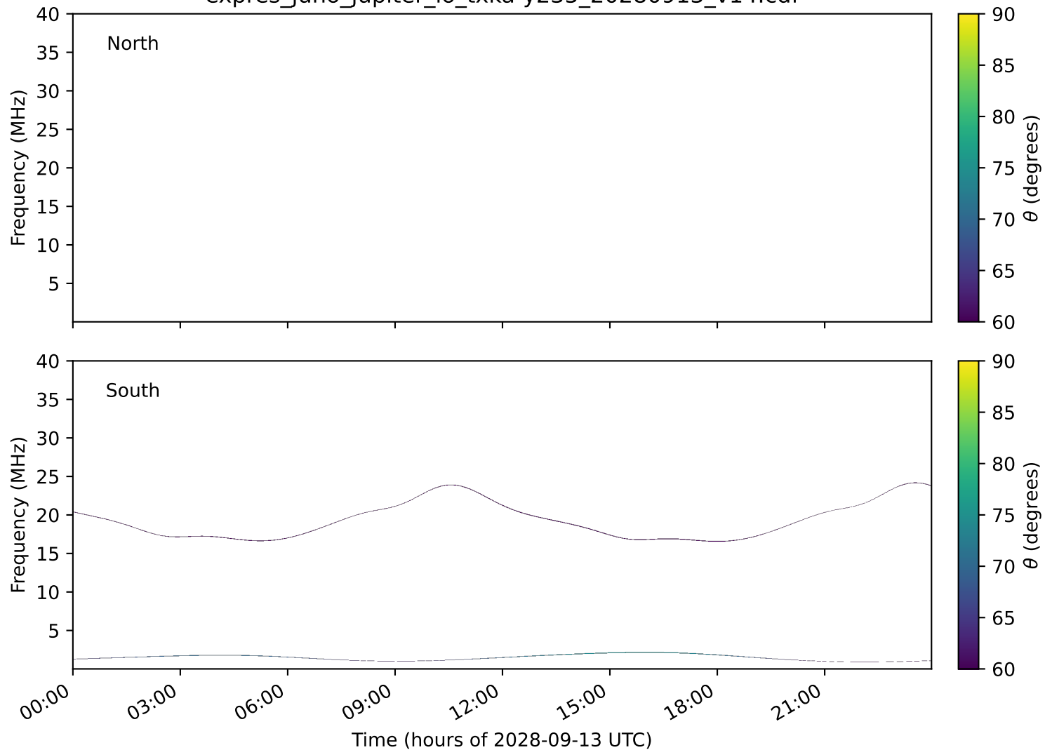
expres_juno_jupiter_io_txka-y235_20280913_v14.cdf
