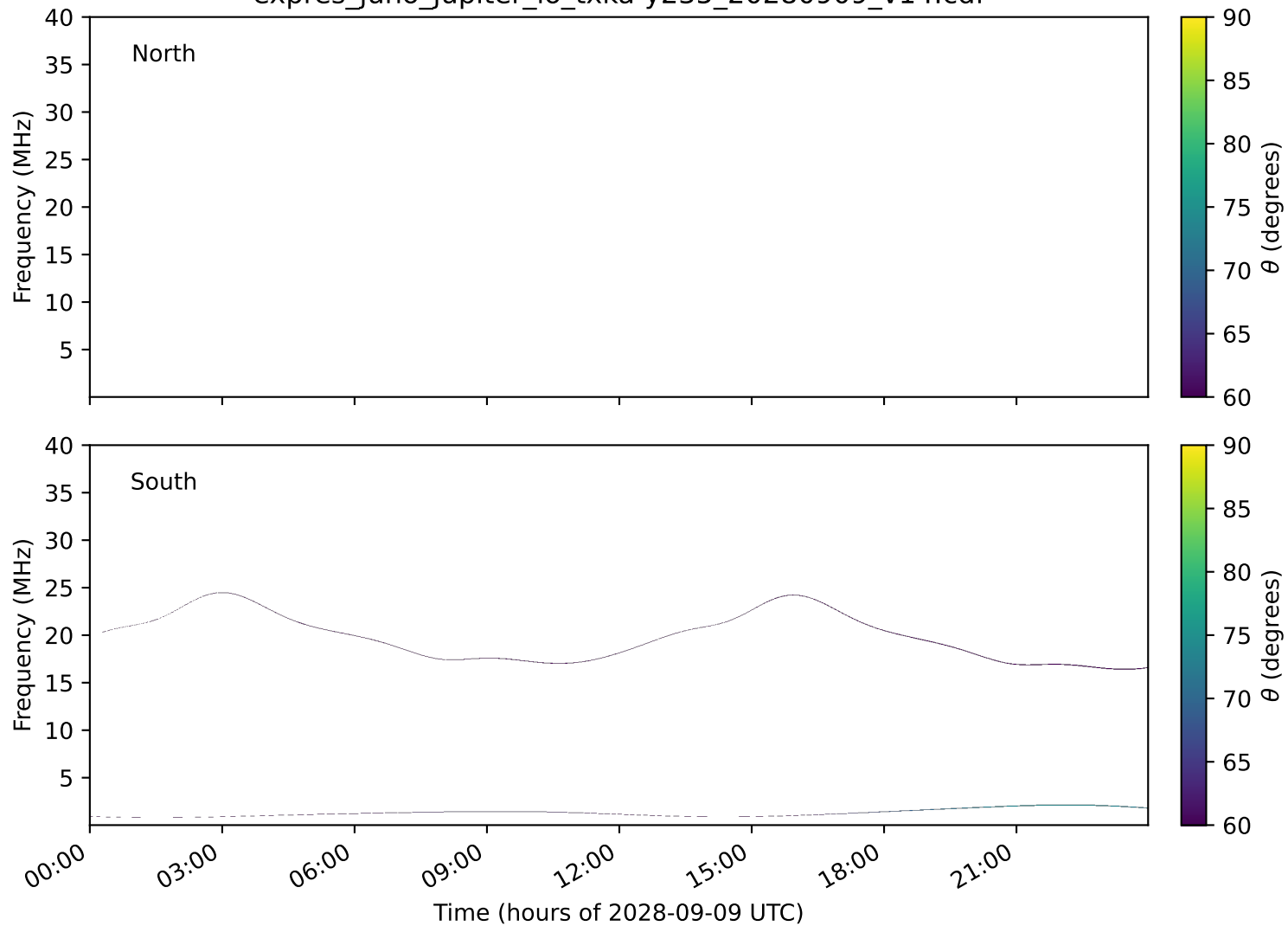
expres_juno_jupiter_io_txka-y235_20280909_v14.cdf
