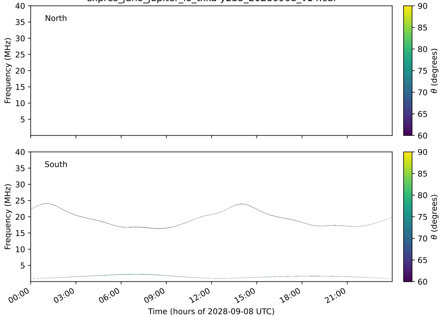
expres_juno_jupiter_io_txka-y235_20280908_v14.cdf
