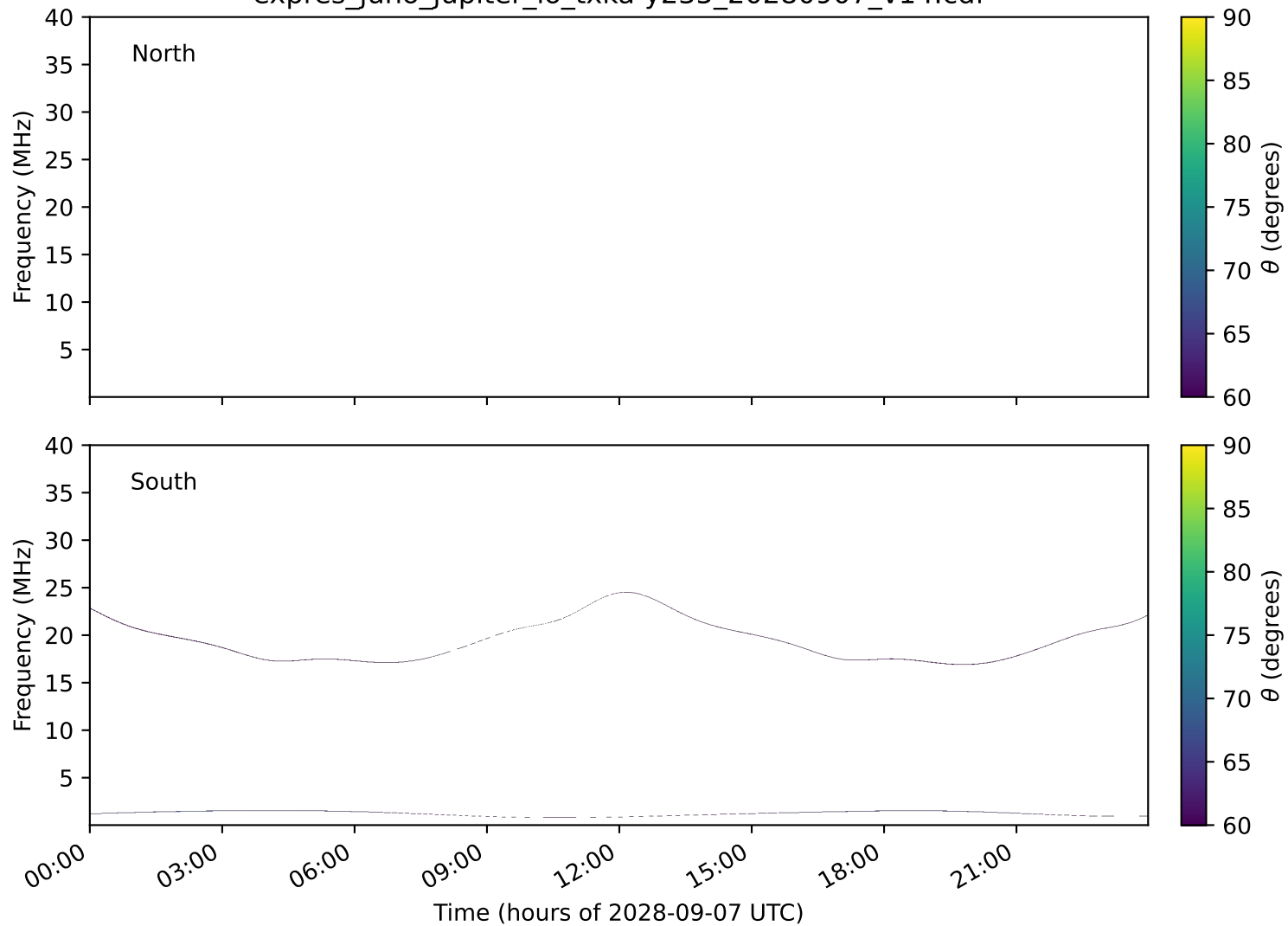
expres_juno_jupiter_io_txka-y235_20280907_v14.cdf
