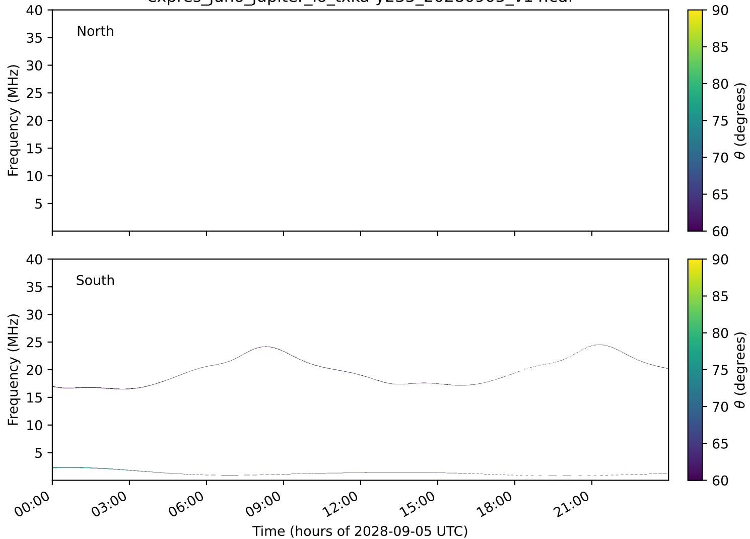
expres_juno_jupiter_io_txka-y235_20280905_v14.cdf
