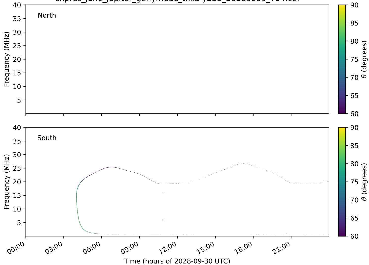
expres_juno_jupiter_ganymede_txka-y235_20280930_v14.cdf
