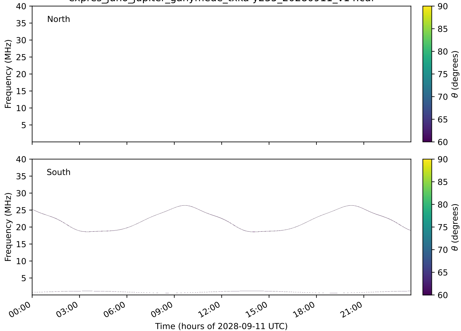
expres_juno_jupiter_ganymede_txka-y235_20280911_v14.cdf
