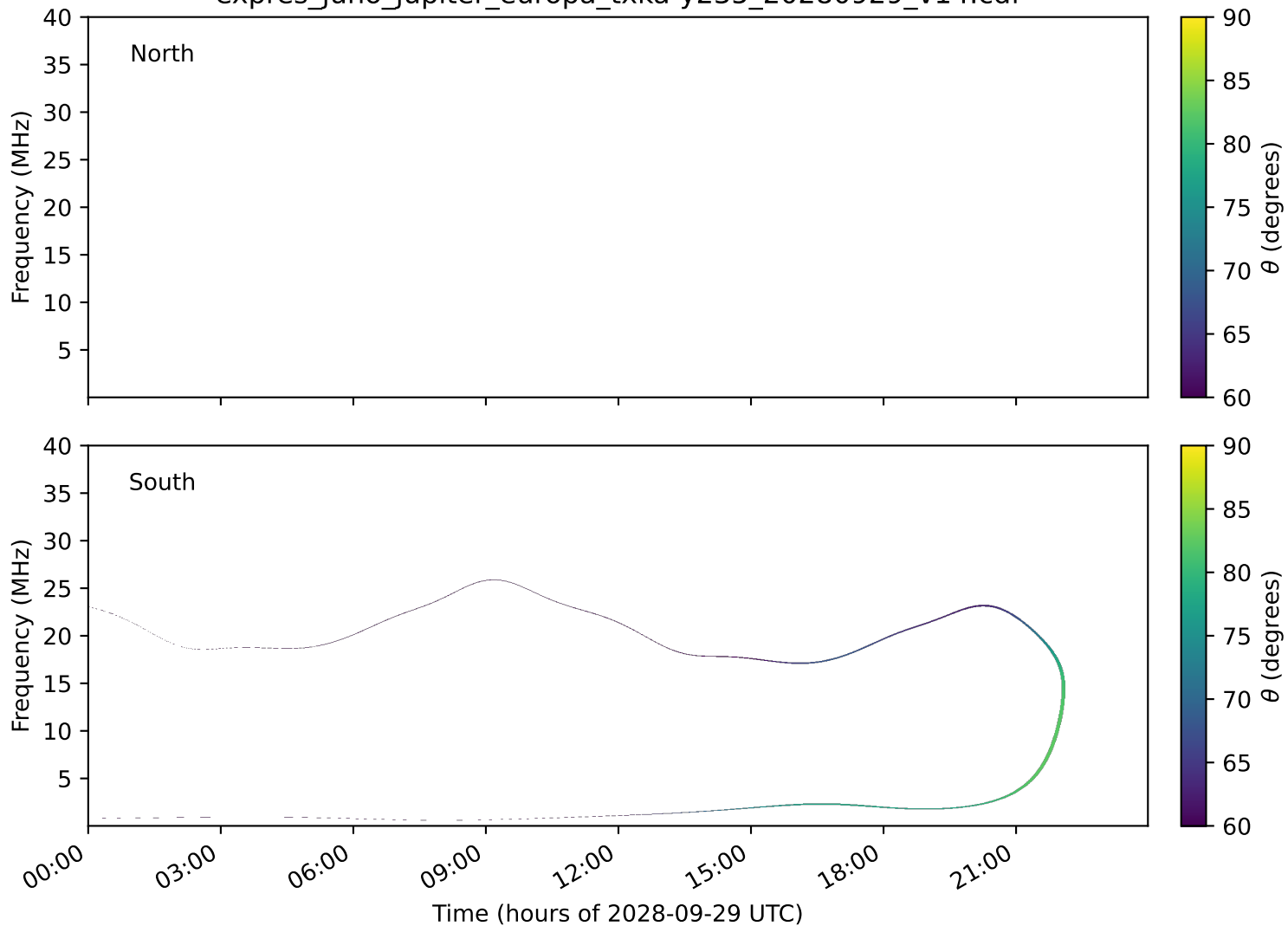
expres_juno_jupiter_europa_txka-y235_20280929_v14.cdf
