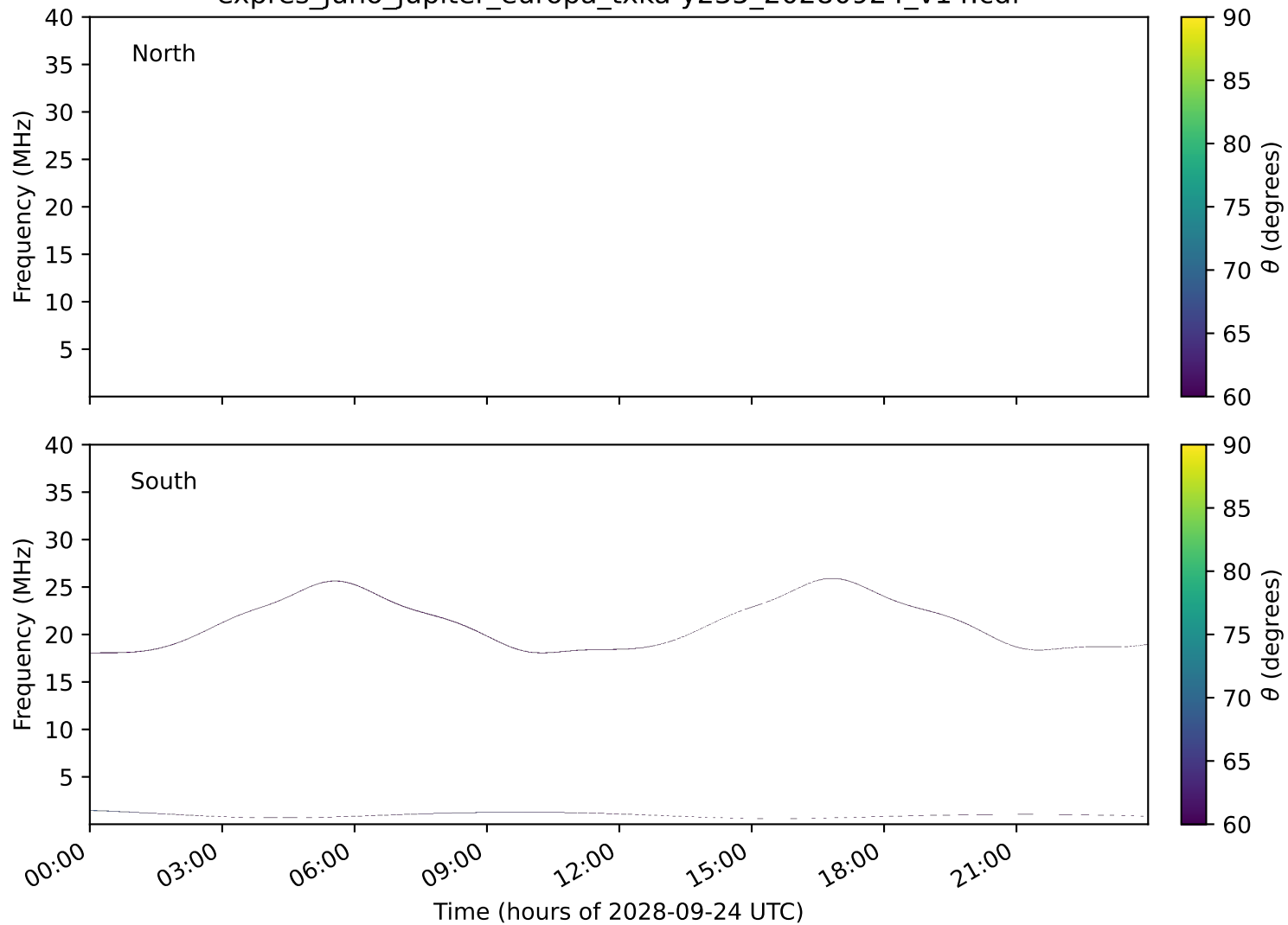
expres_juno_jupiter_europa_txka-y235_20280924_v14.cdf
