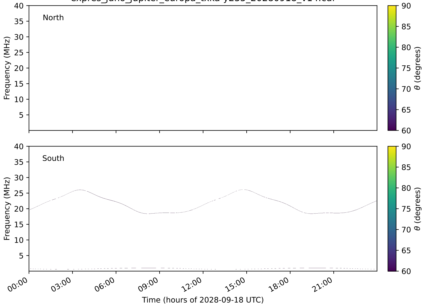
expres_juno_jupiter_europa_txka-y235_20280918_v14.cdf
