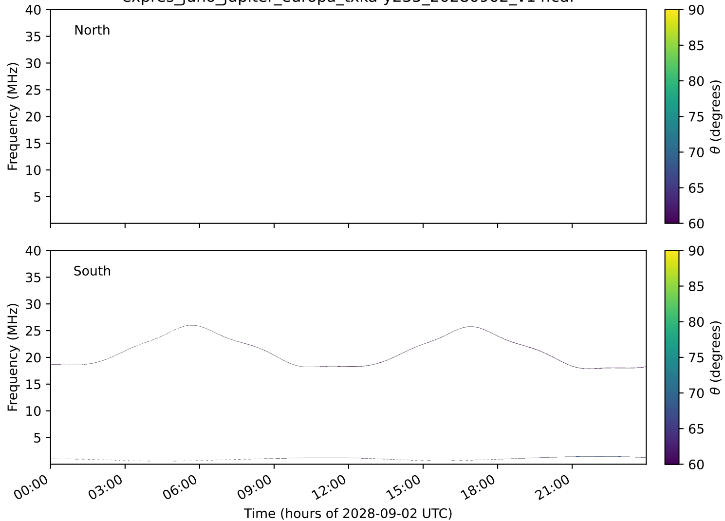
expres_juno_jupiter_europa_txka-y235_20280902_v14.cdf
