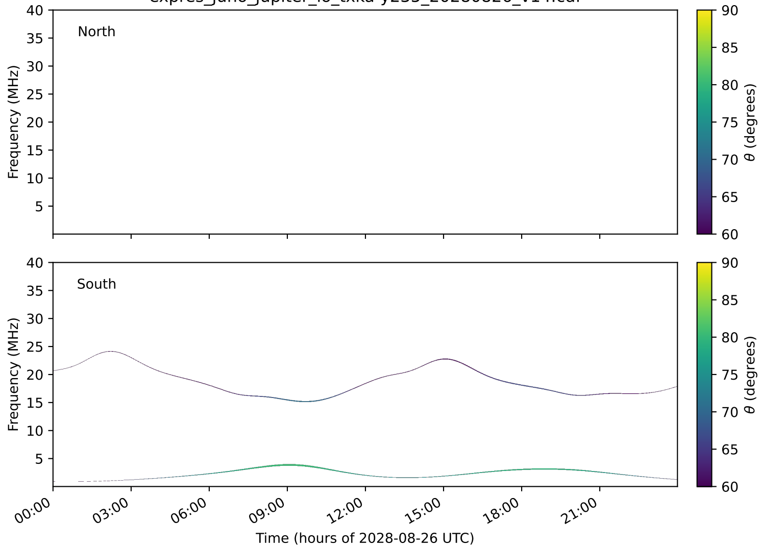
expres_juno_jupiter_io_txka-y235_20280826_v14.cdf
