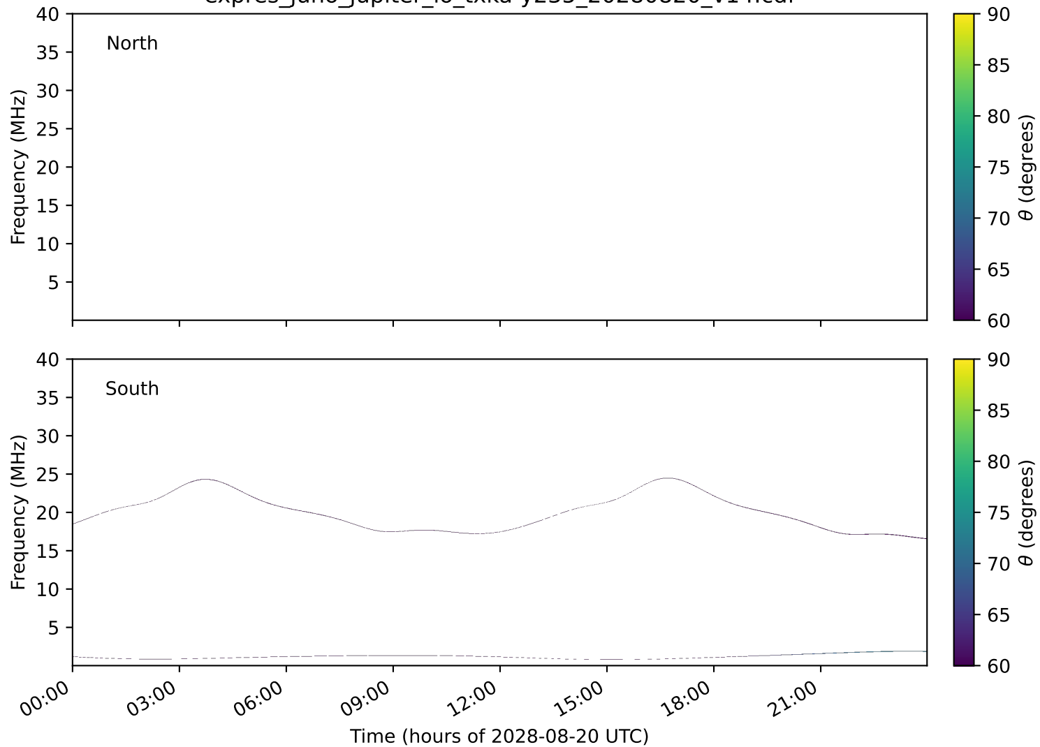
expres_juno_jupiter_io_txka-y235_20280820_v14.cdf
