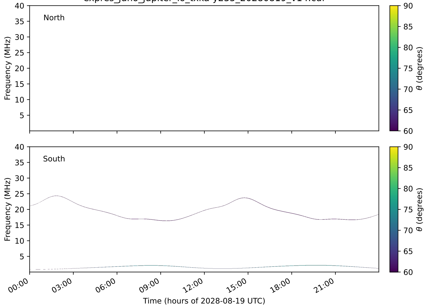
expres_juno_jupiter_io_txka-y235_20280819_v14.cdf
