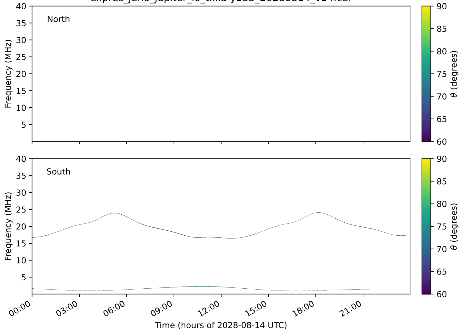
expres_juno_jupiter_io_txka-y235_20280814_v14.cdf
