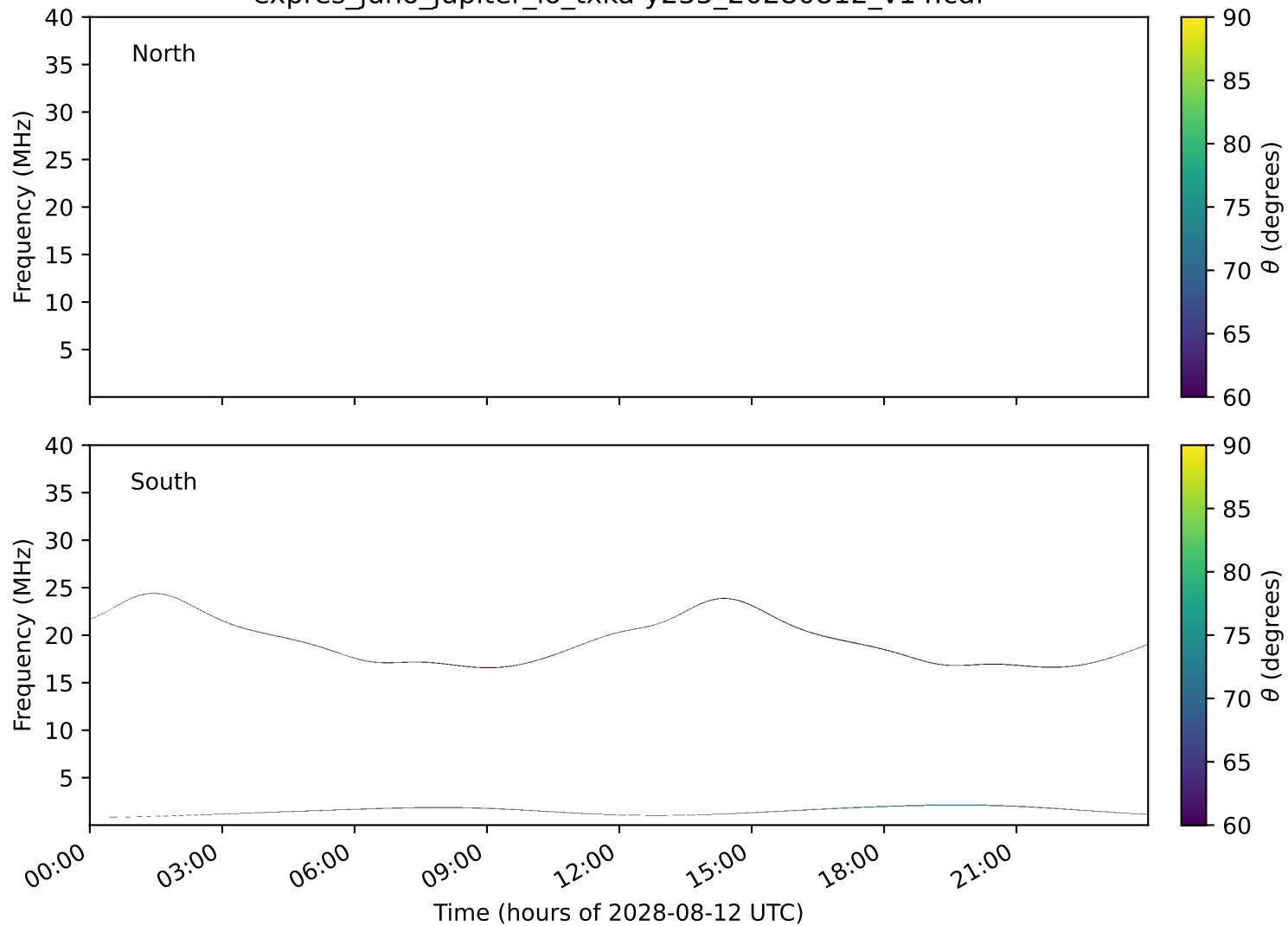
expres_juno_jupiter_io_txka-y235_20280812_v14.cdf
