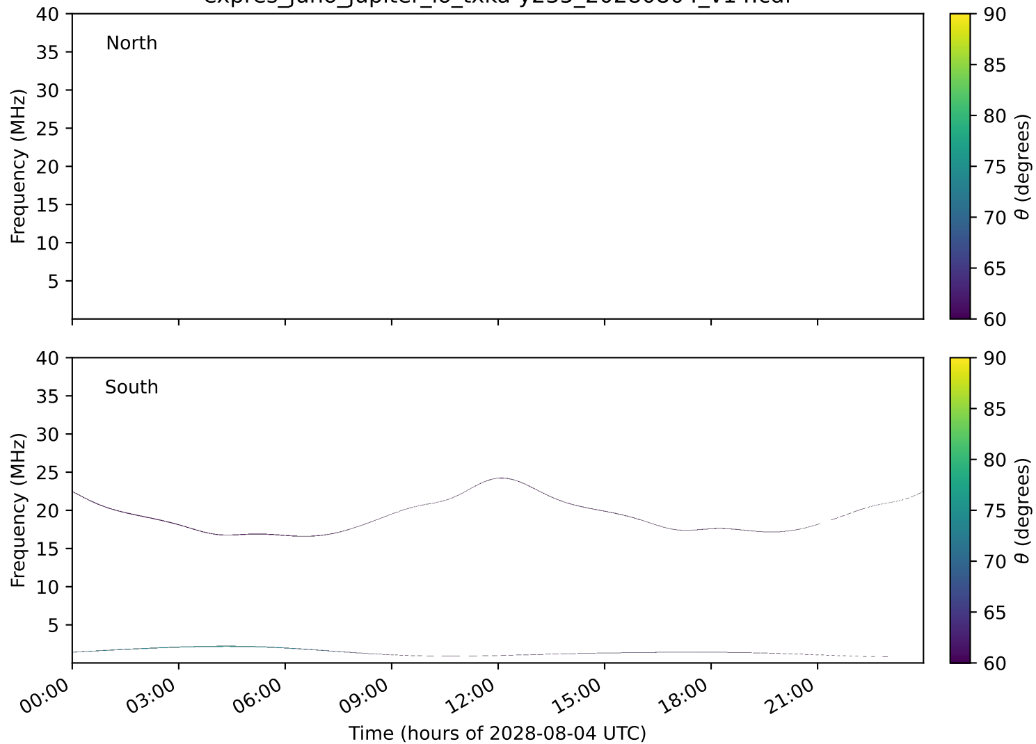
expres_juno_jupiter_io_txka-y235_20280804_v14.cdf
