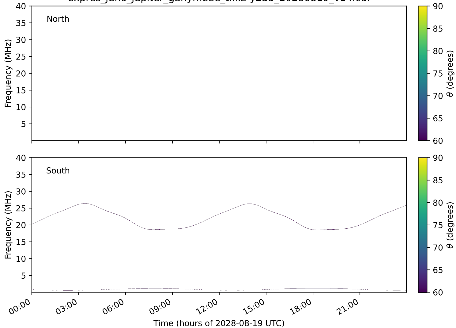
expres_juno_jupiter_ganymede_txka-y235_20280819_v14.cdf
