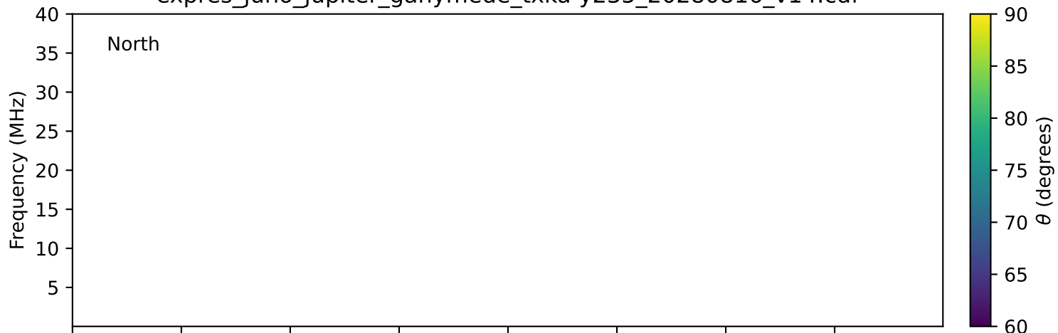
expres_juno_jupiter_ganymede_txka-y235_20280816_v14.cdf
