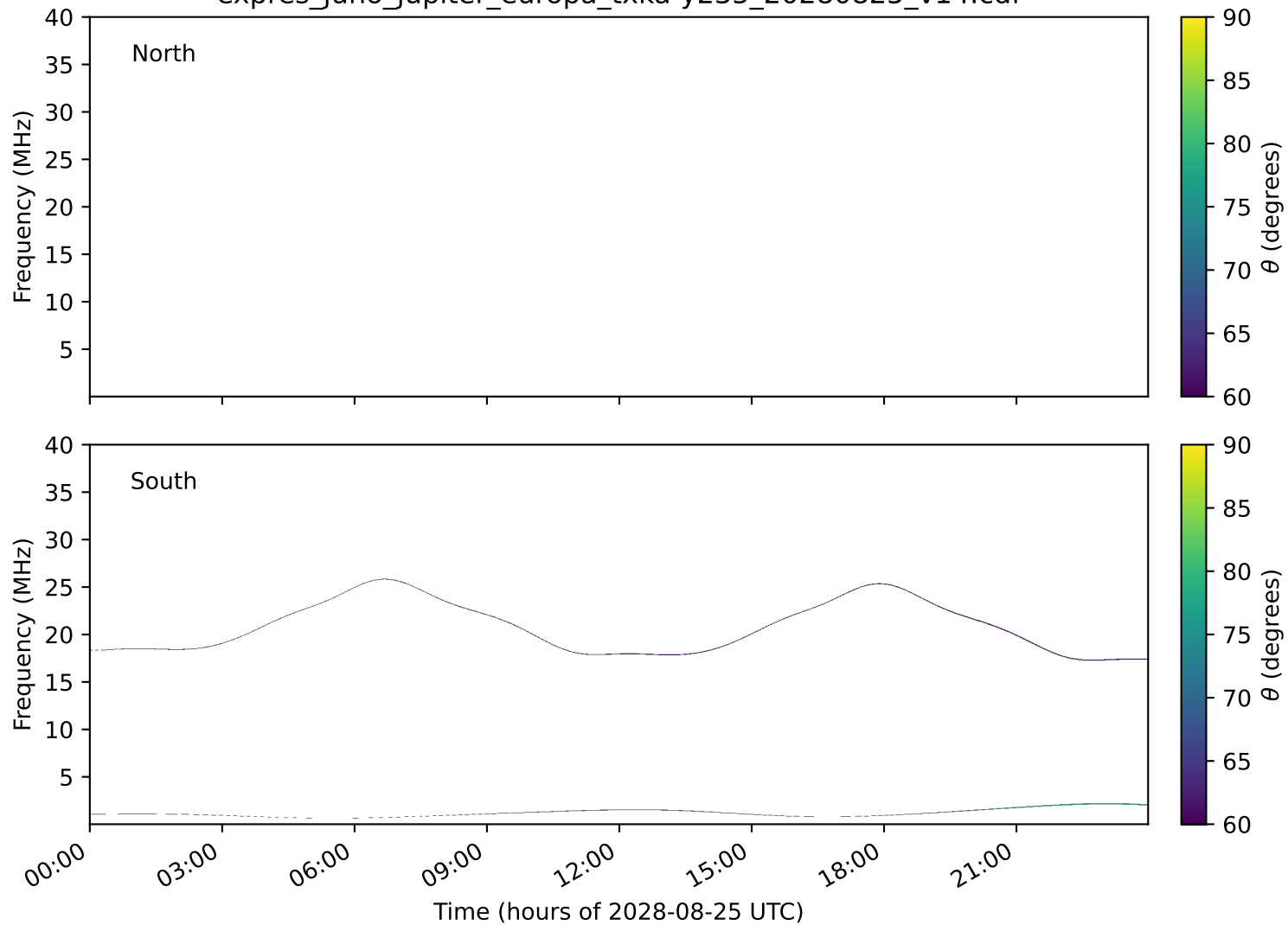
expres_juno_jupiter_europa_txka-y235_20280825_v14.cdf
