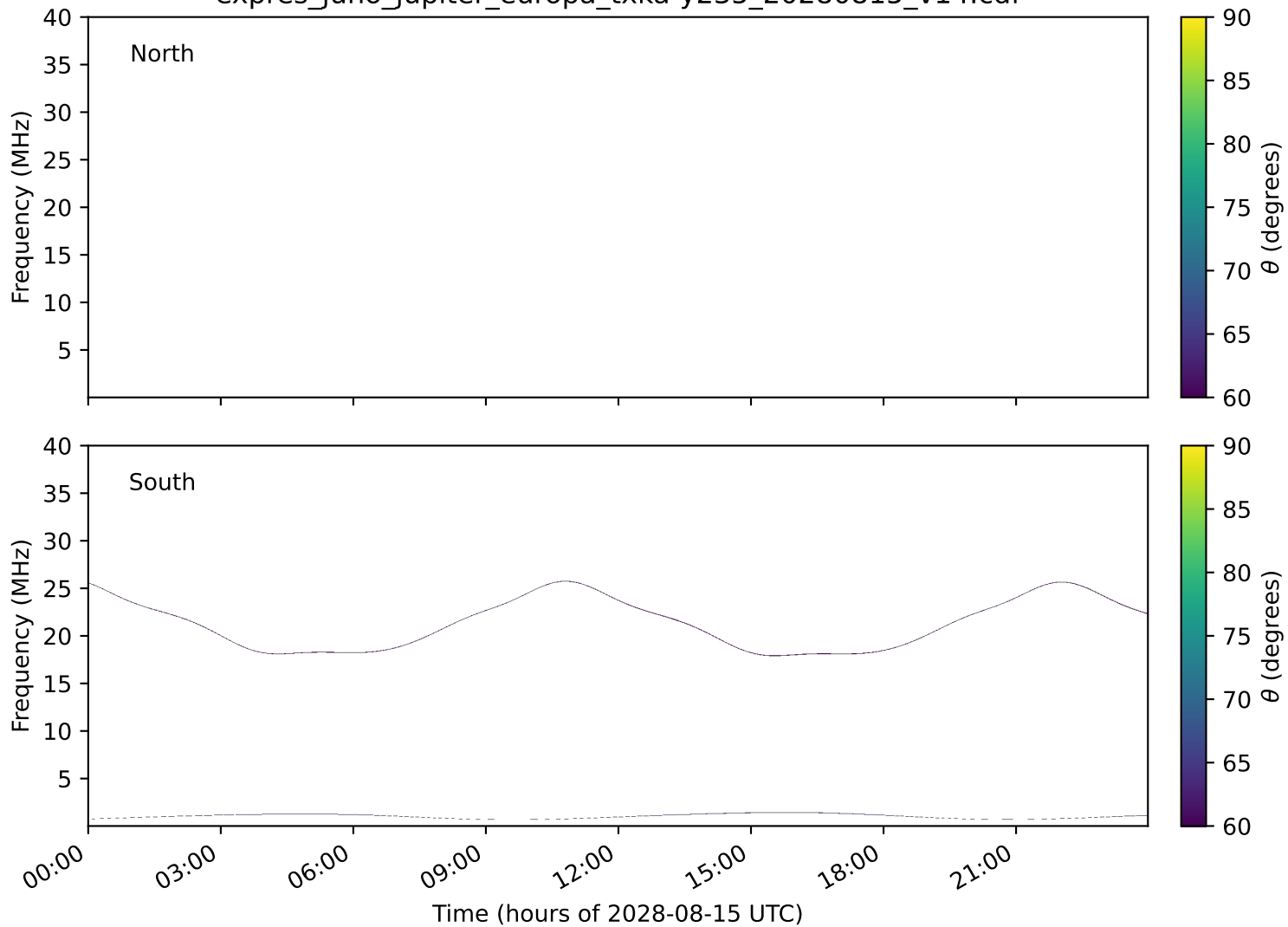
expres_juno_jupiter_europa_txka-y235_20280815_v14.cdf
