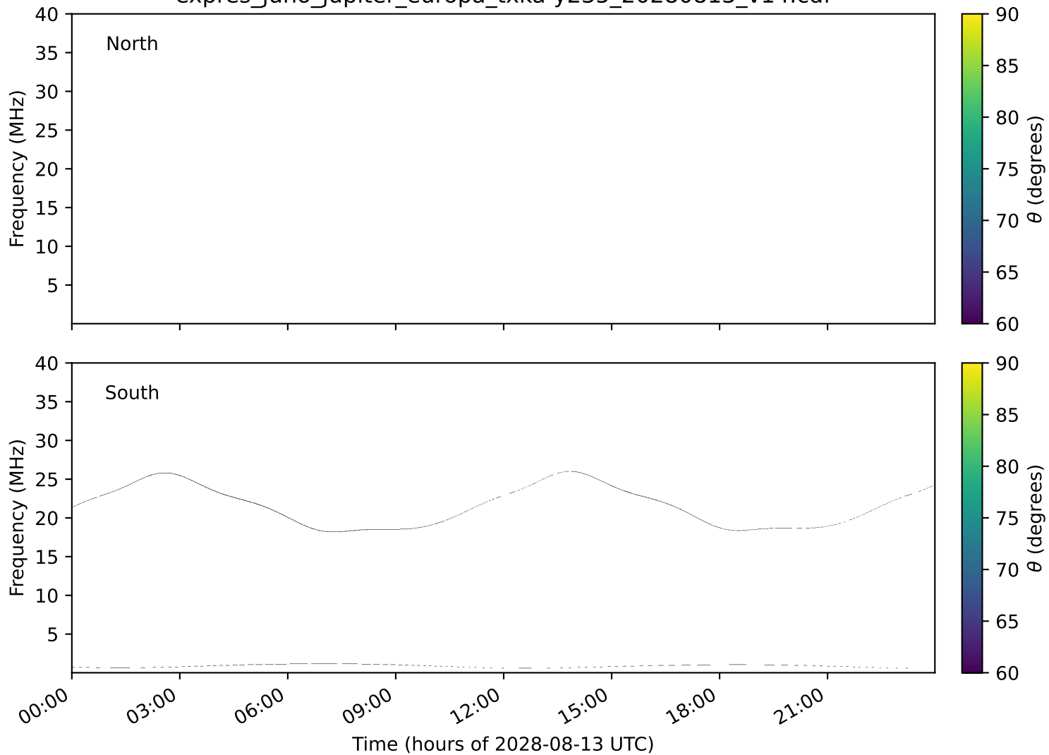
expres_juno_jupiter_europa_txka-y235_20280813_v14.cdf
