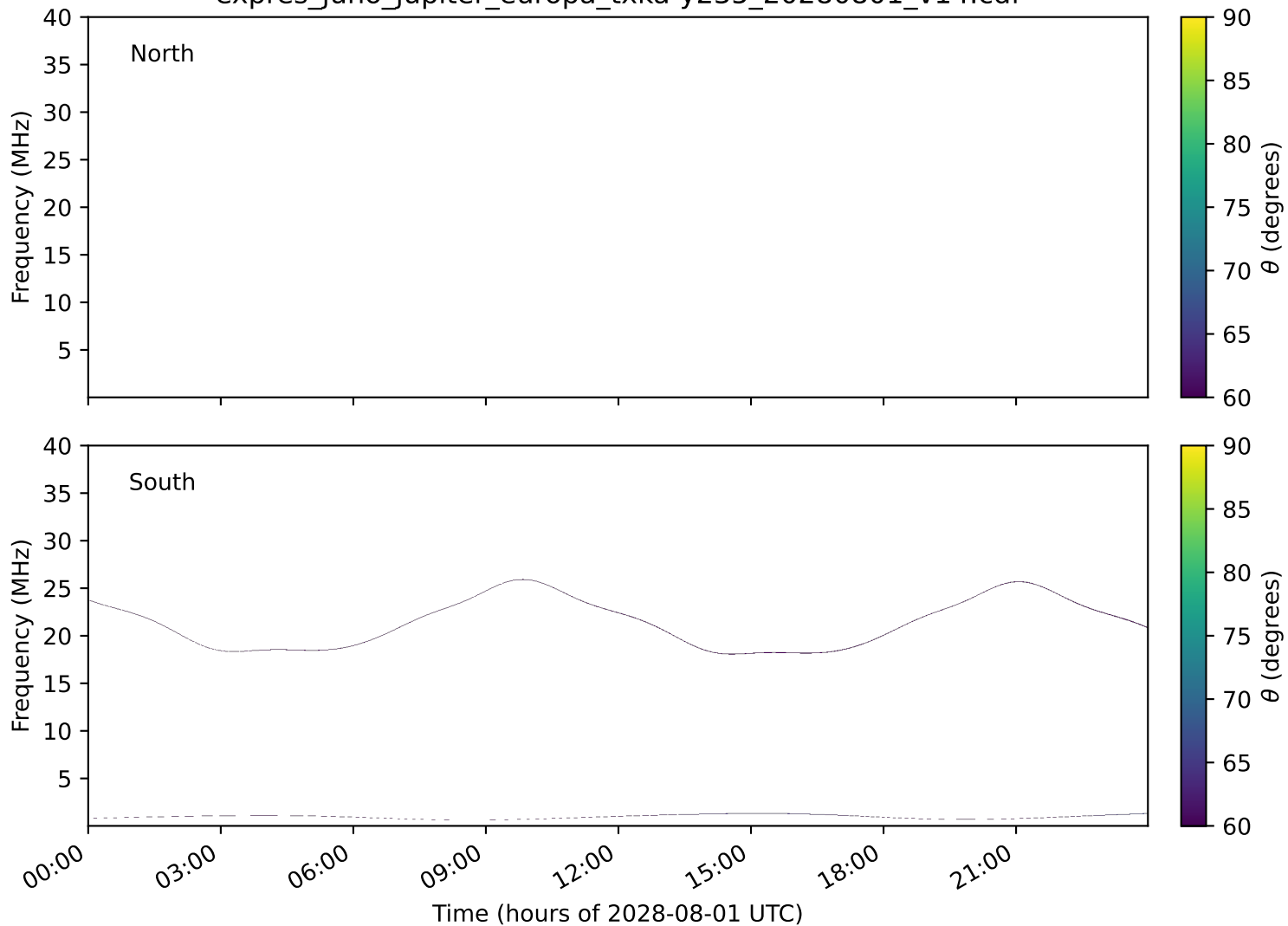
expres_juno_jupiter_europa_txka-y235_20280801_v14.cdf
