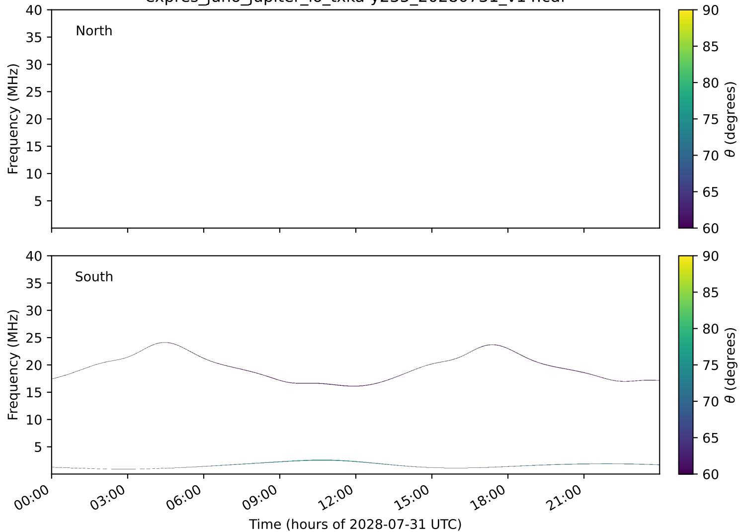
expres_juno_jupiter_io_txka-y235_20280731_v14.cdf
