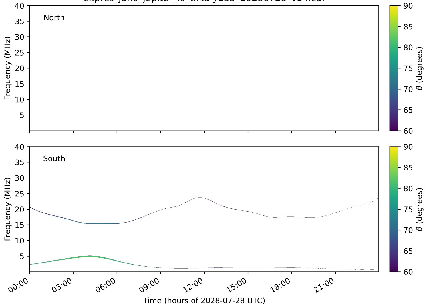
expres_juno_jupiter_io_txka-y235_20280728_v14.cdf
