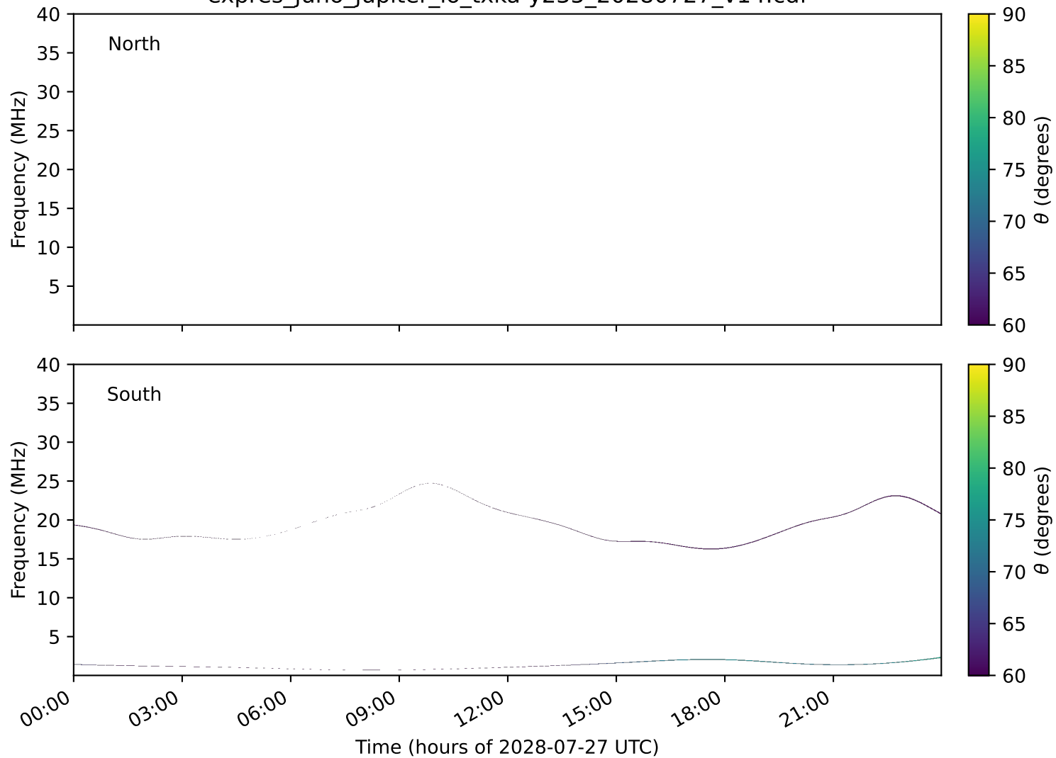
expres_juno_jupiter_io_txka-y235_20280727_v14.cdf
