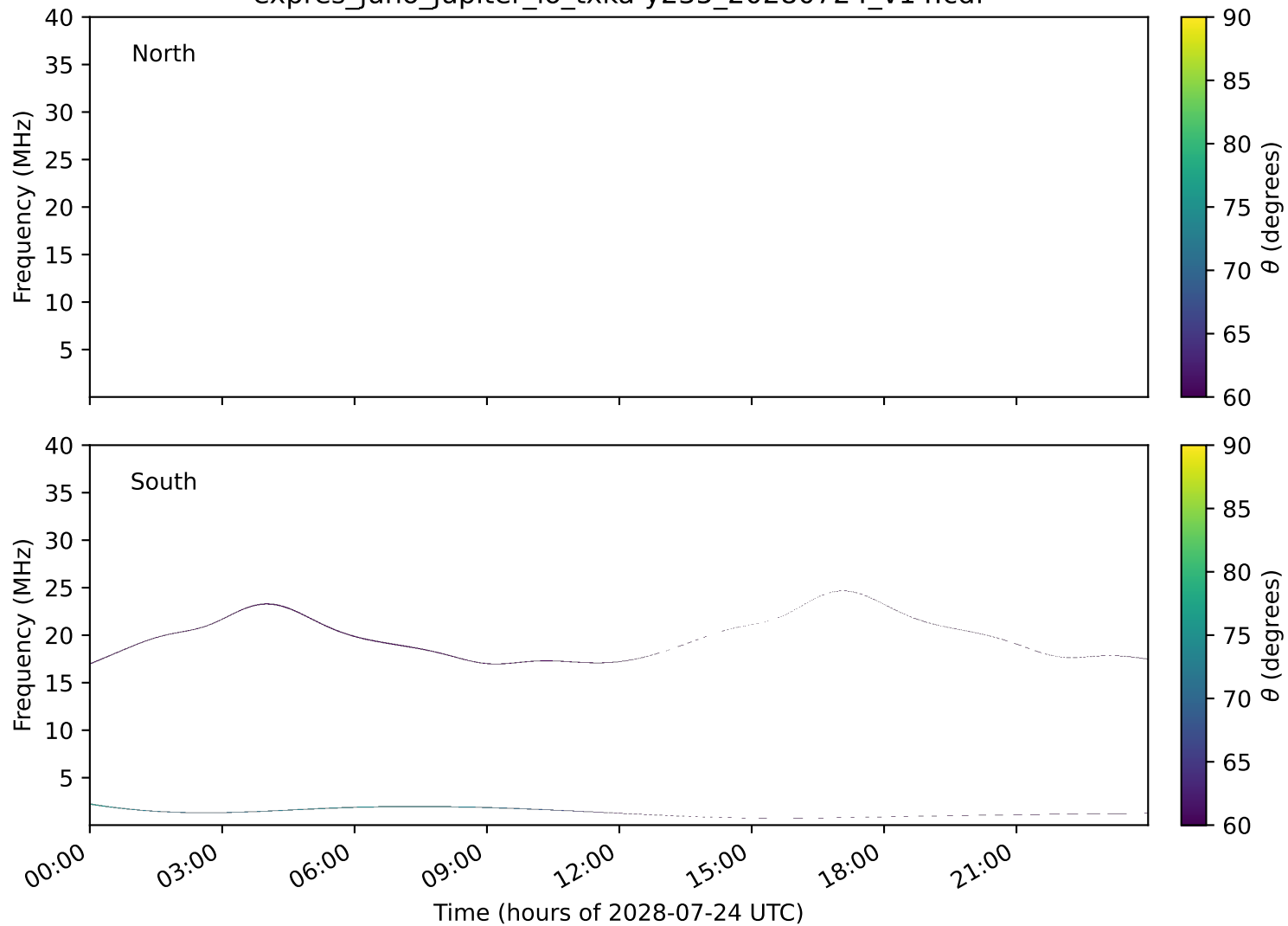
expres_juno_jupiter_io_txka-y235_20280724_v14.cdf
