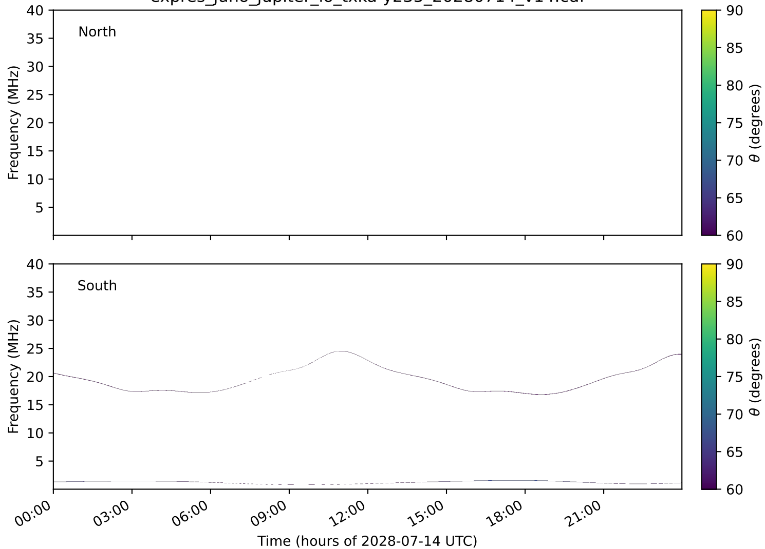
expres_juno_jupiter_io_txka-y235_20280714_v14.cdf
