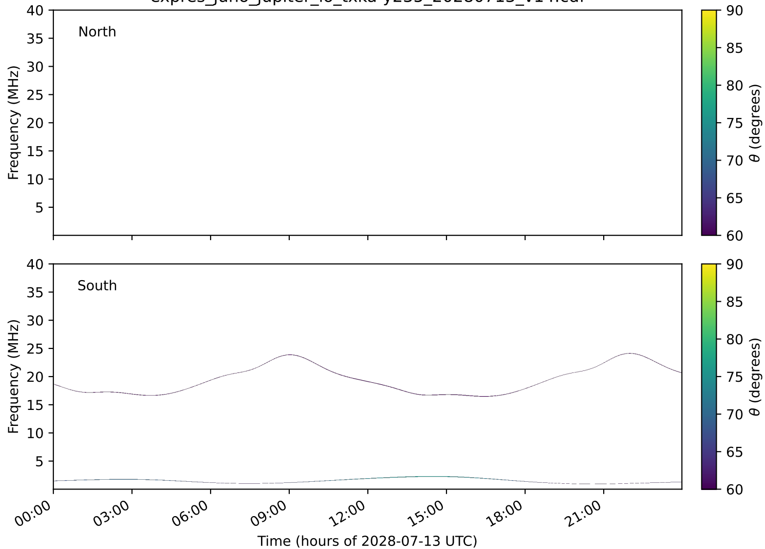
expres_juno_jupiter_io_txka-y235_20280713_v14.cdf
