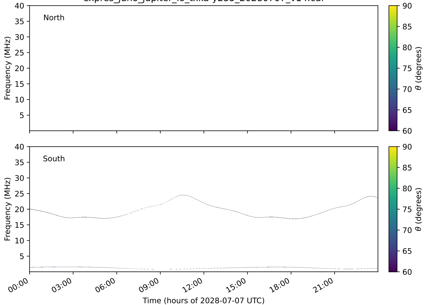
expres_juno_jupiter_io_txka-y235_20280707_v14.cdf
