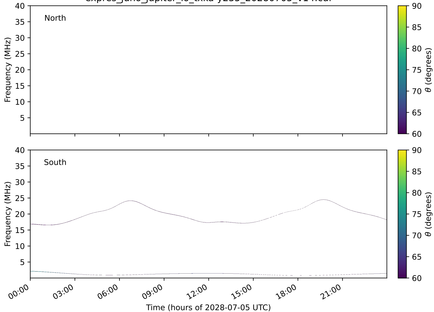
expres_juno_jupiter_io_txka-y235_20280705_v14.cdf
