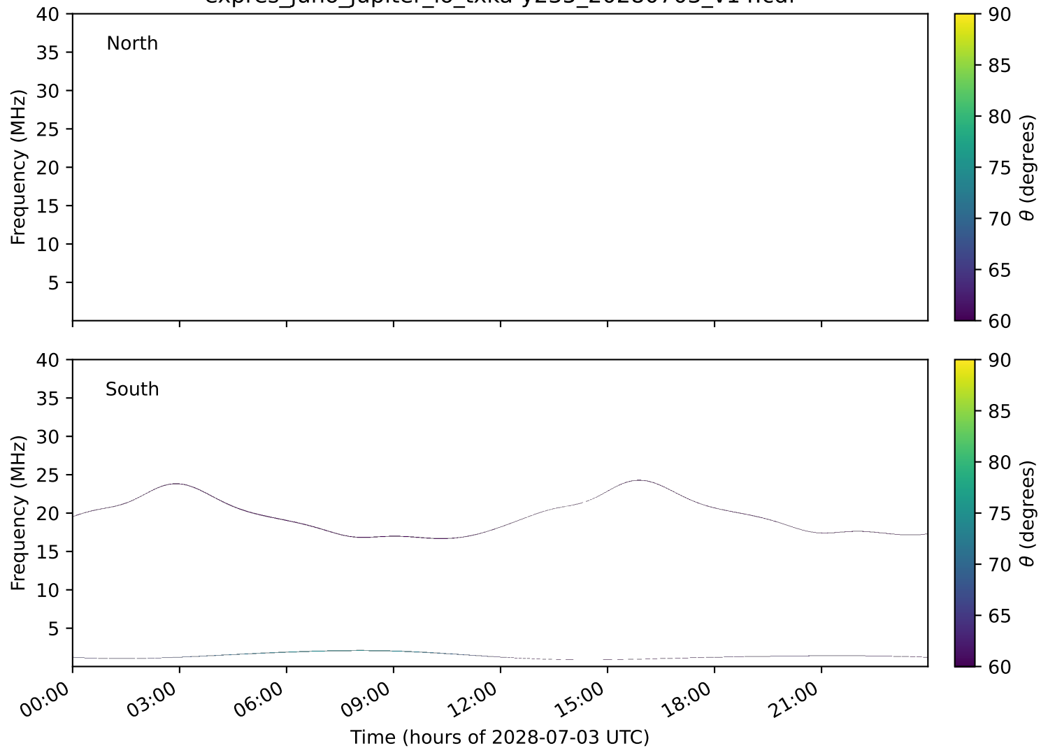
expres_juno_jupiter_io_txka-y235_20280703_v14.cdf
