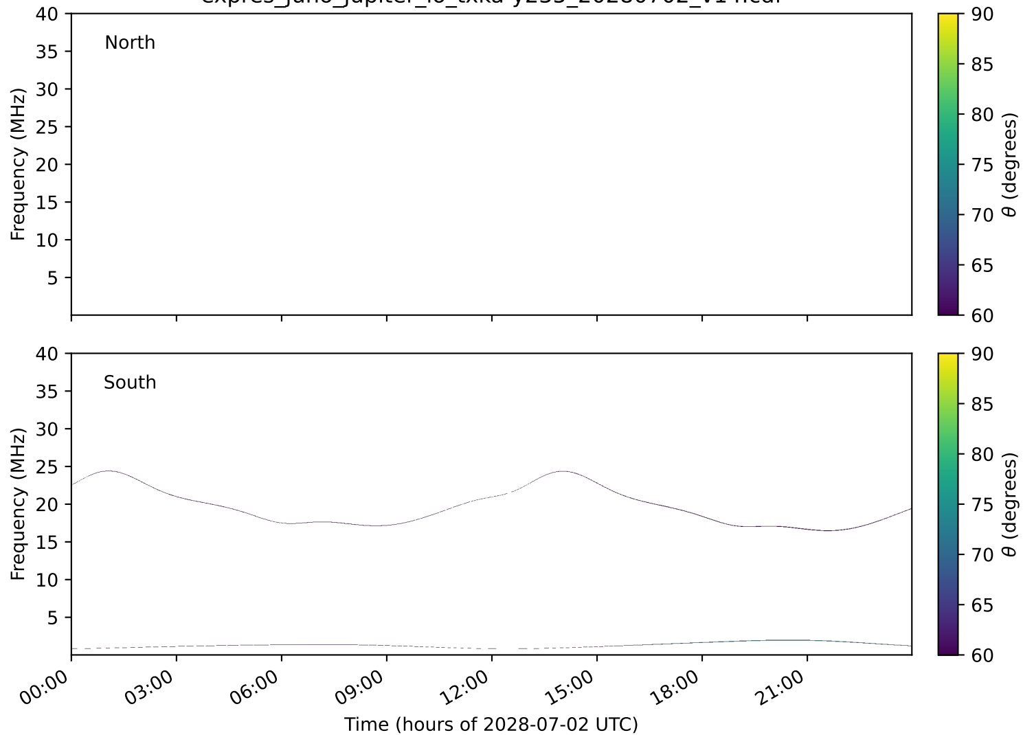
expres_juno_jupiter_io_txka-y235_20280702_v14.cdf
