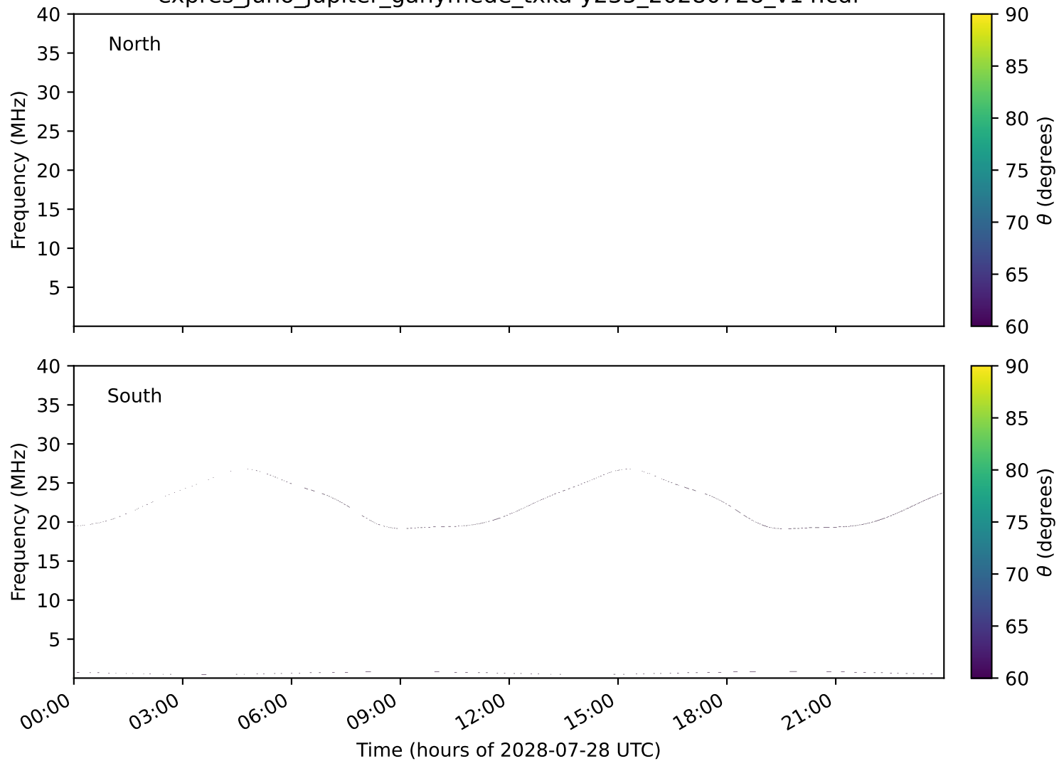
expres_juno_jupiter_ganymede_txka-y235_20280728_v14.cdf
