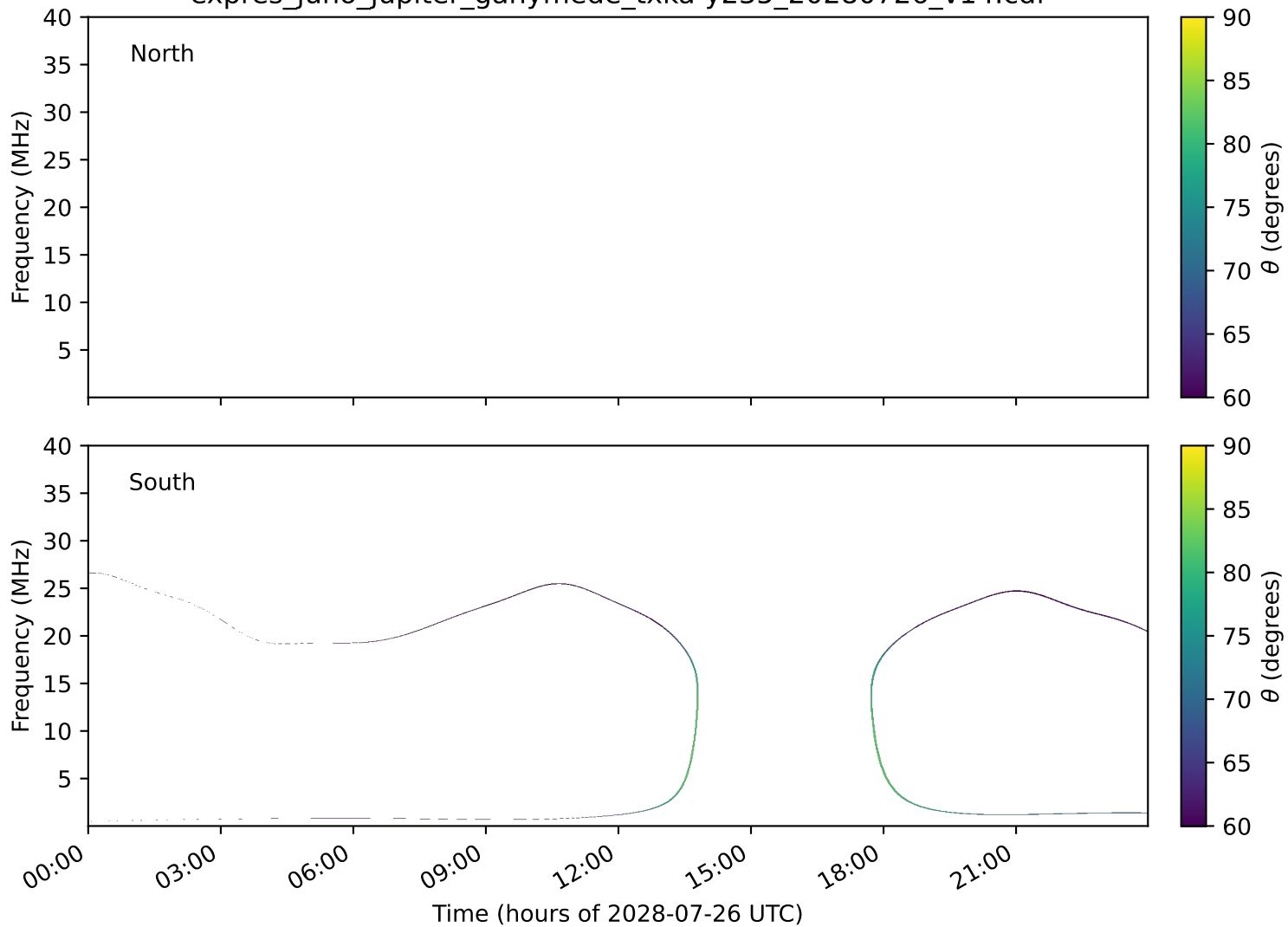
expres_juno_jupiter_ganymede_txka-y235_20280726_v14.cdf
