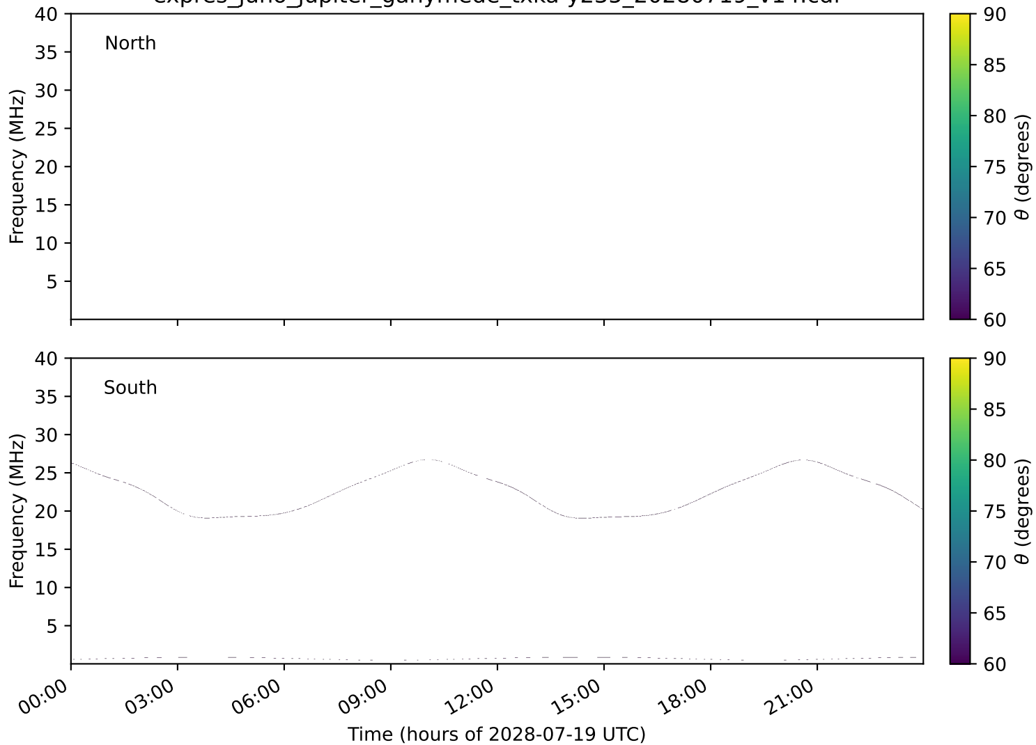
expres_juno_jupiter_ganymede_txka-y235_20280719_v14.cdf
